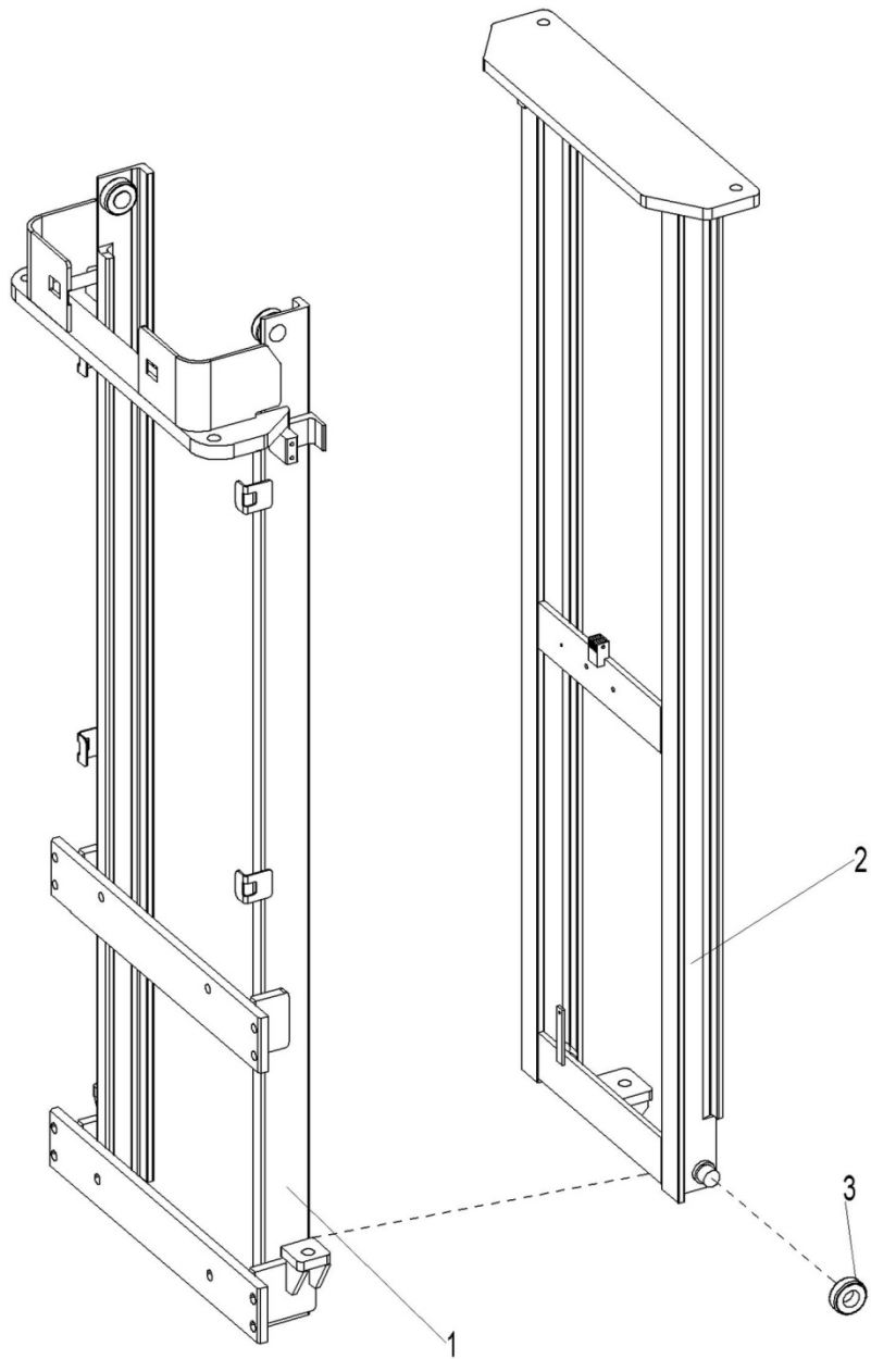
Fig. 9 Two-stage mast system (full free lift)
