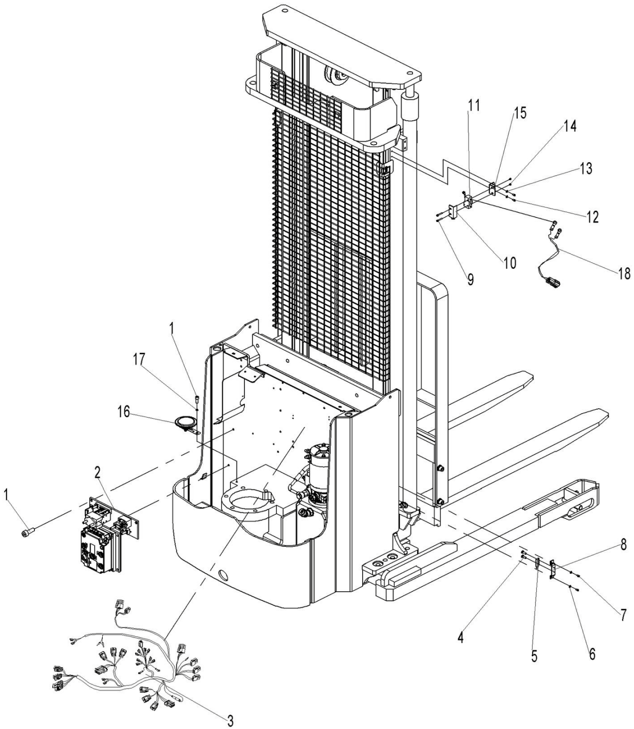
Fig. 25 Electrical parts
