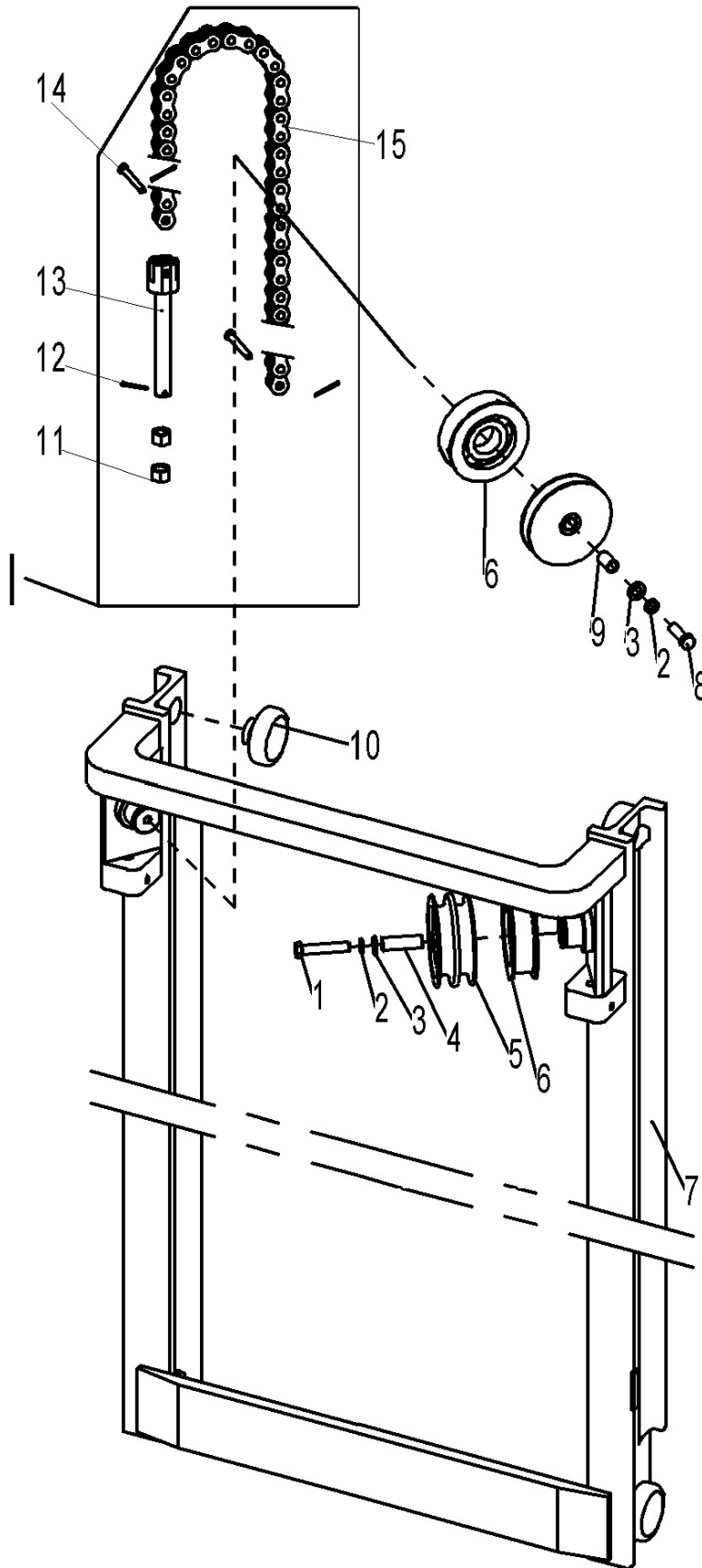
Fig. 15 Middle mast kits (three stage mast)
