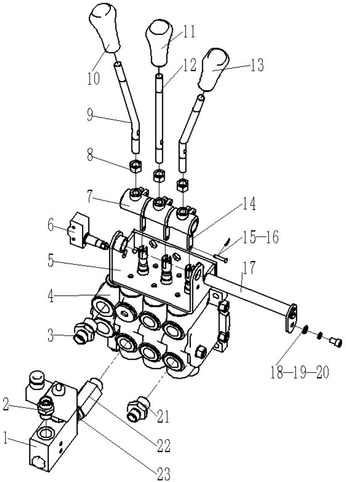
Fig.40 Multi-tandem valve (three ways)
