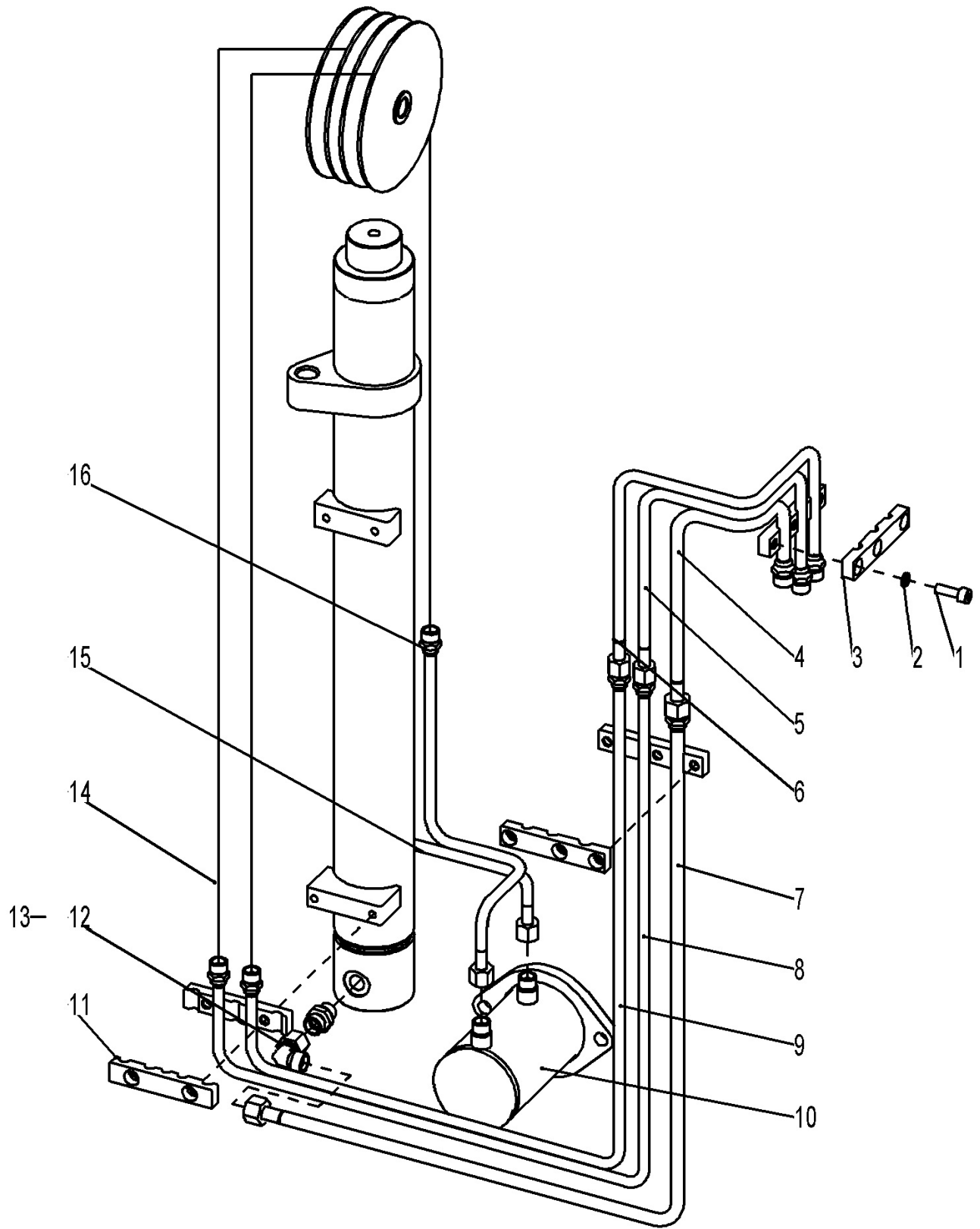
Fig. 17 Single mast hydraulic pipeline (three ways)
