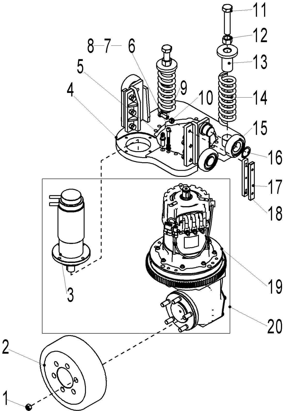
Fig. 23 Drive assembly
