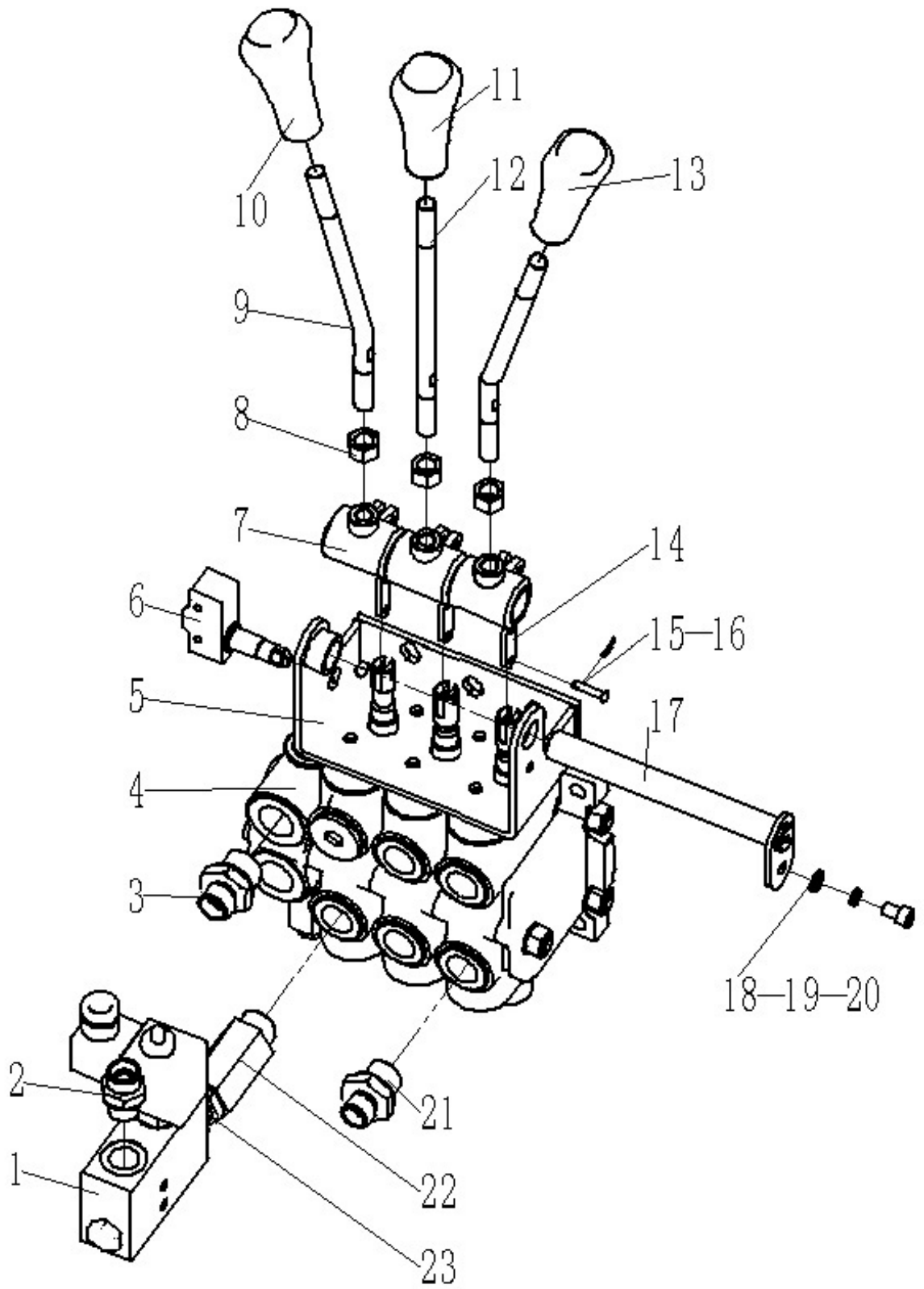
Fig. 40 Multi tandem valve (three ways)
