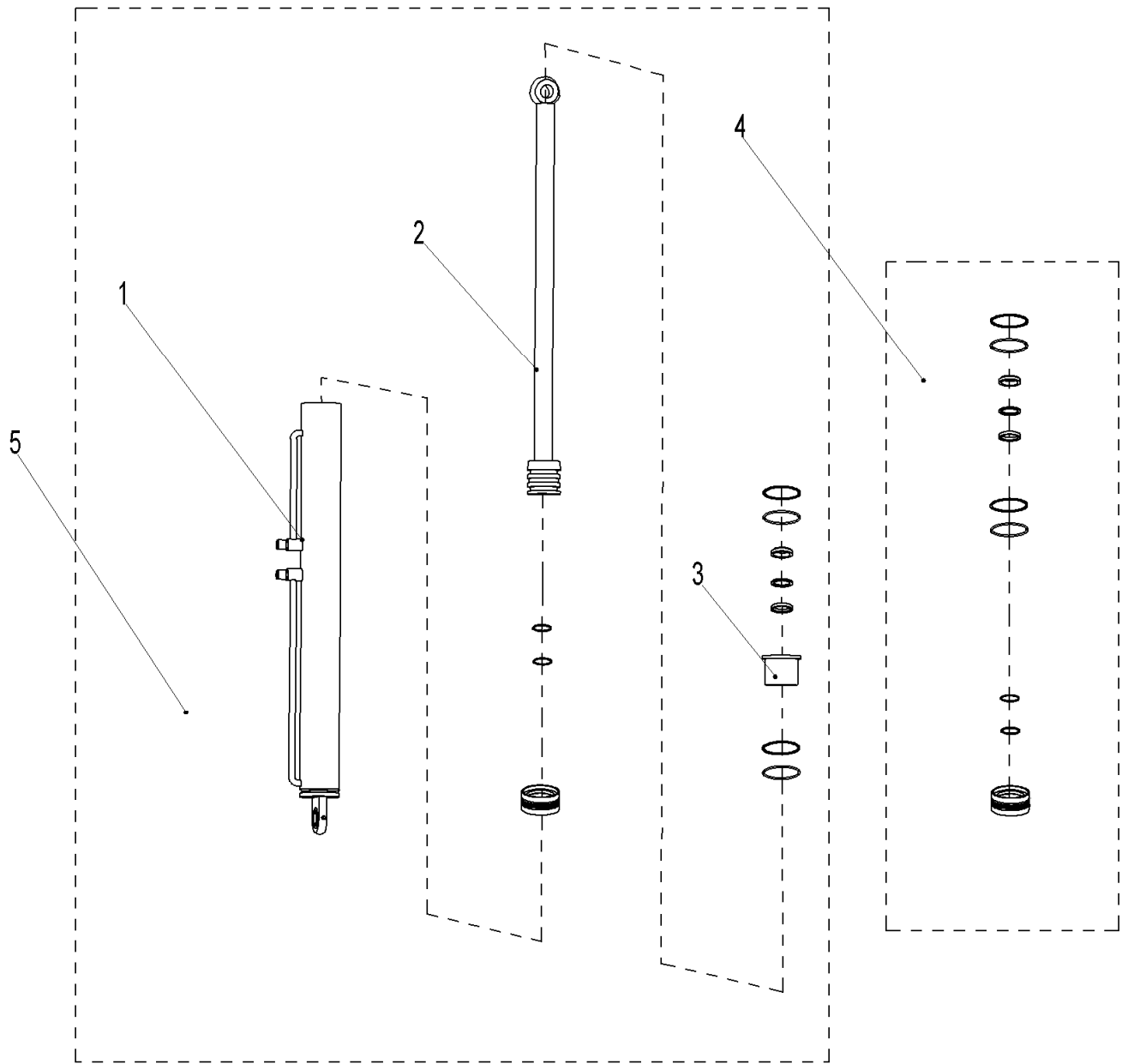
Fig. 37 Forward cylinder
