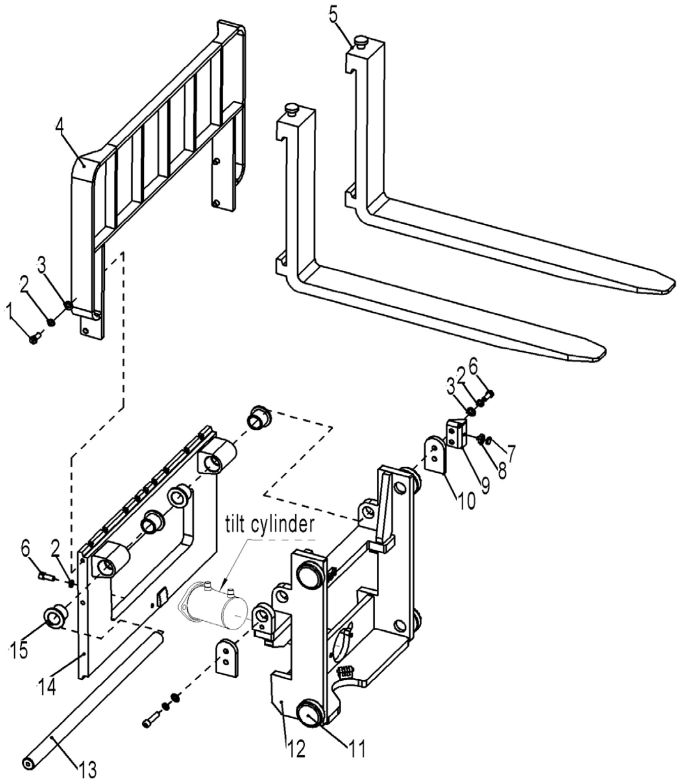
Fig. 11 Fork frame kits (three-stage-mast)
