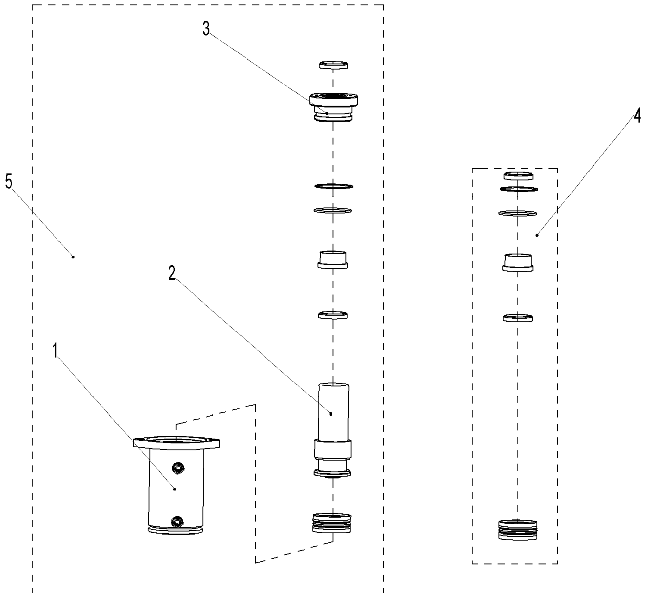
Fig. 32 Tilt cylinder
