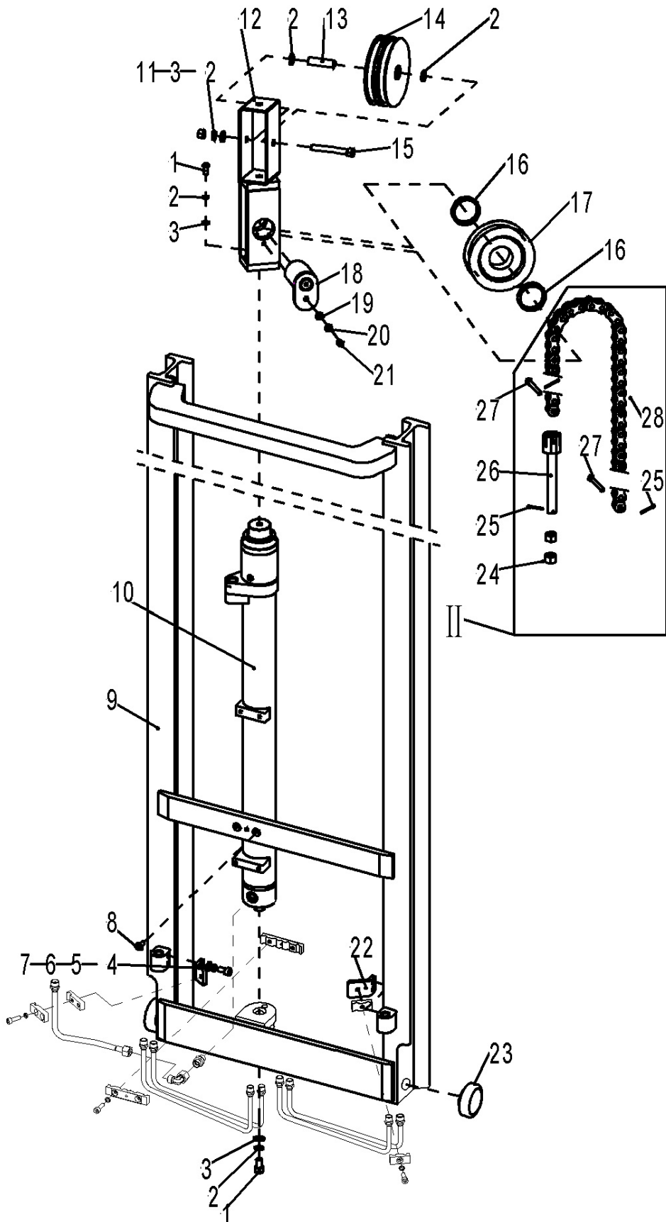
Fig. 16 Inner mast kits (three stage mast)
