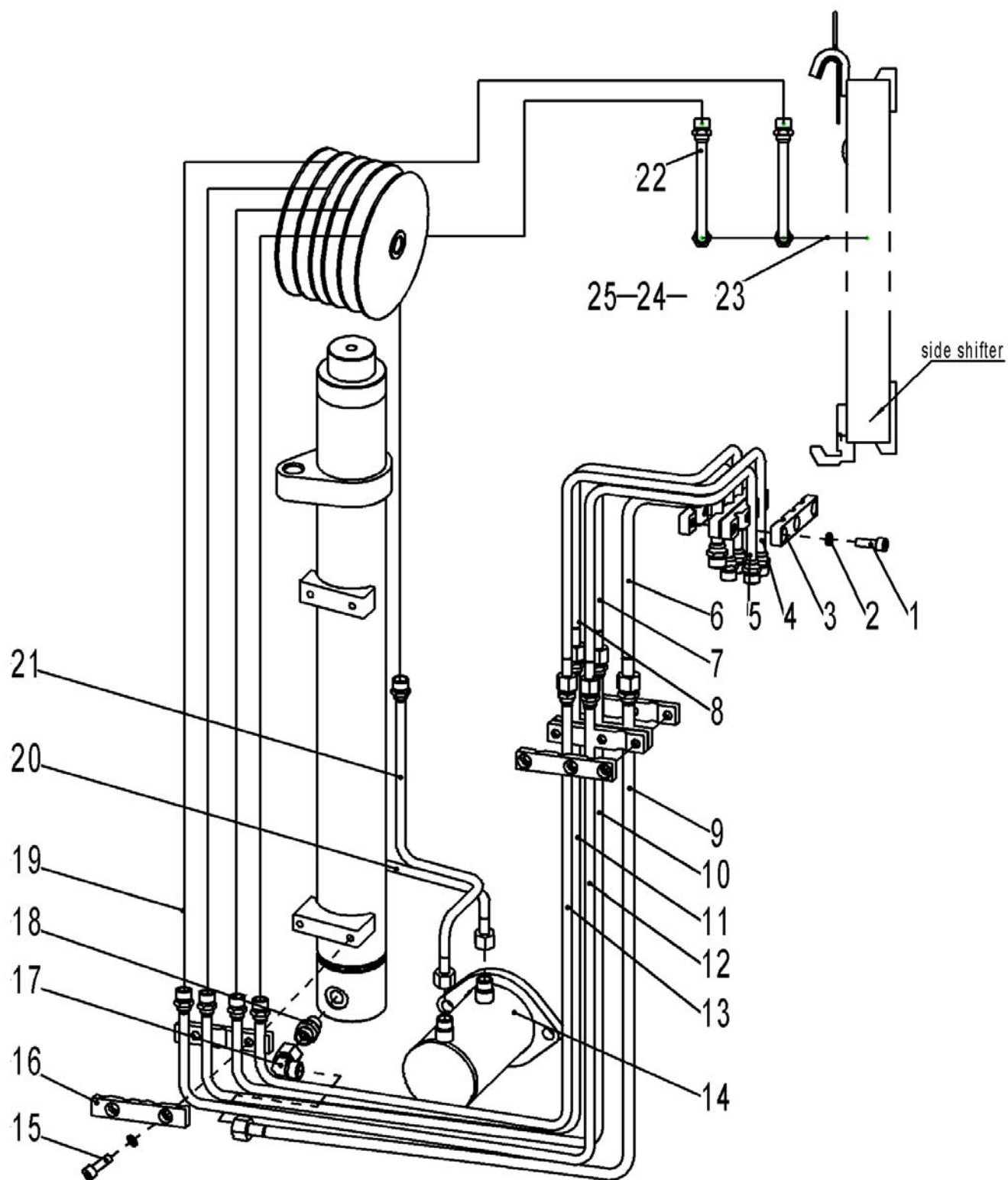
Fig. 18 Single mast hydraulic pipeline (four ways)
