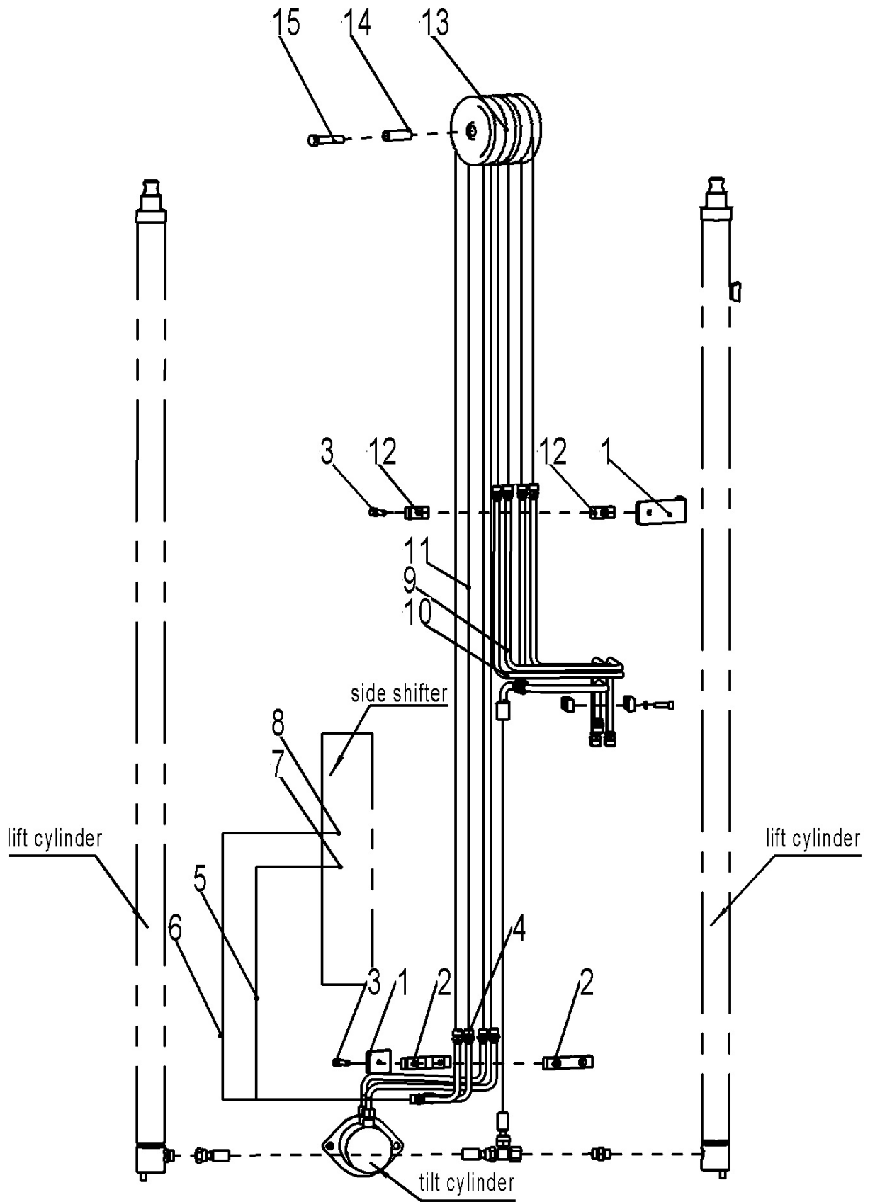
Fig. 20 Two stage mast hydraulic pipeline (four ways)
