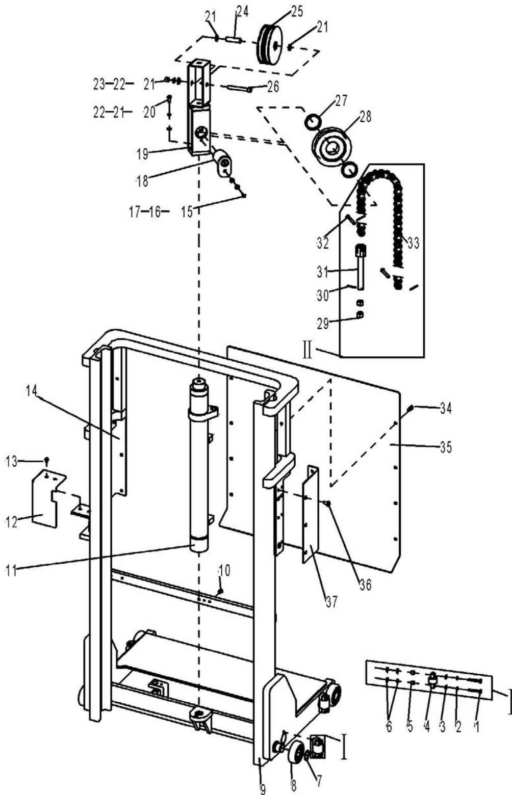
Fig. 12 Outer mast kits (single mast)
