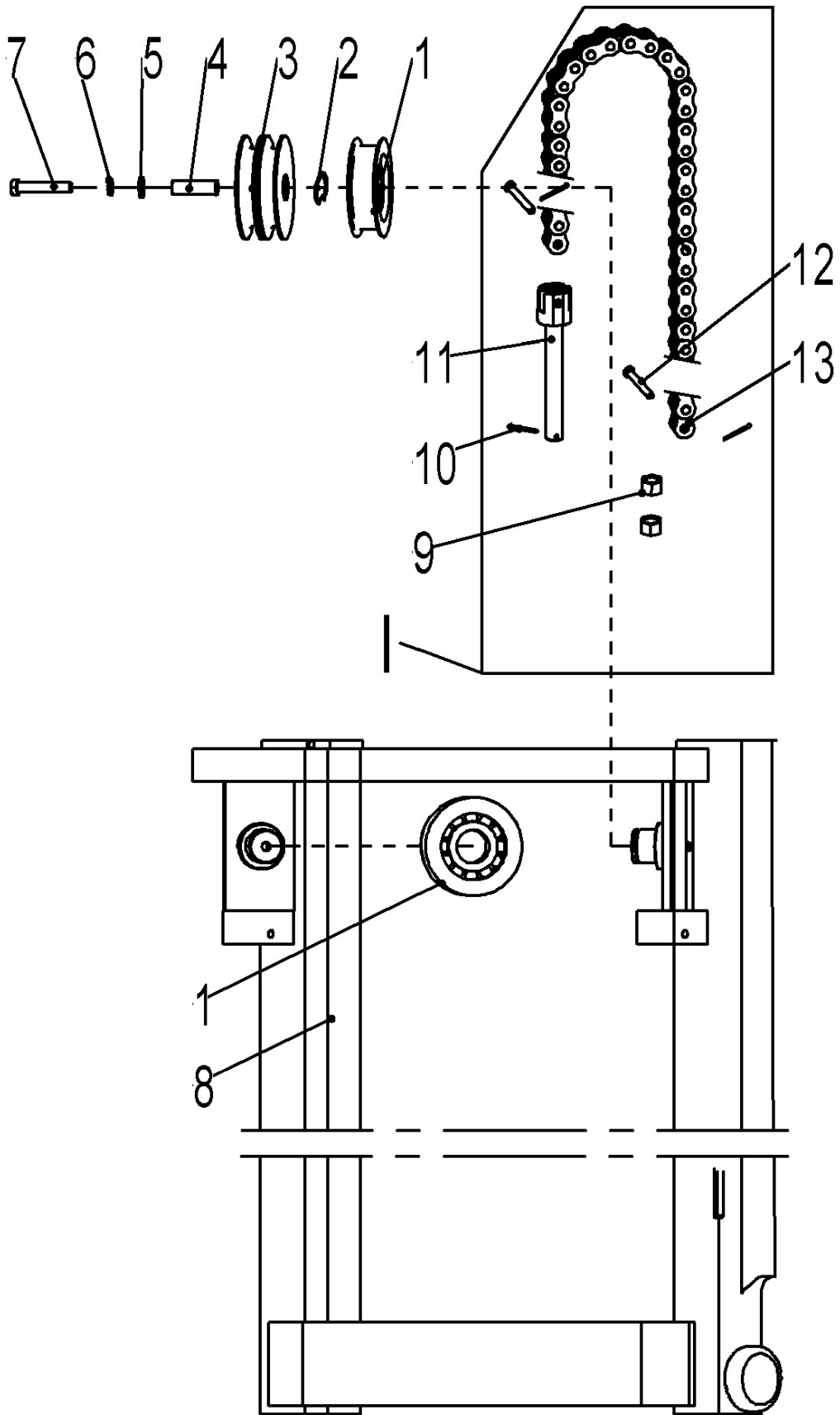
Fig. 14 Inner mast kits (Two stage mast)
