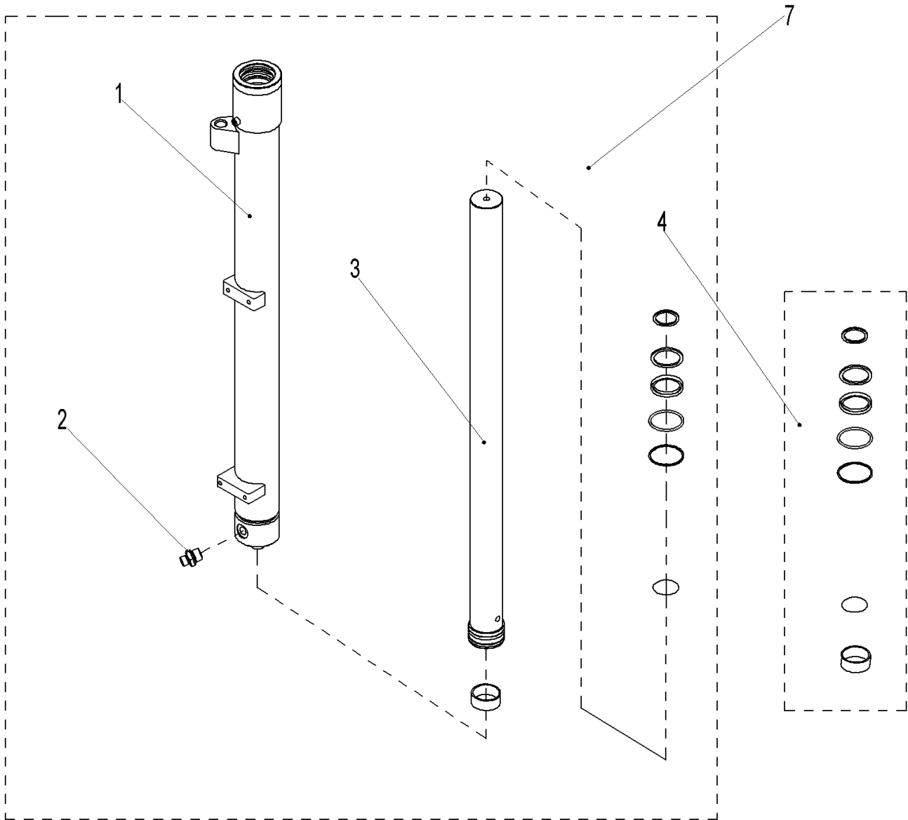
Fig. 38 Front lifting cylinder
