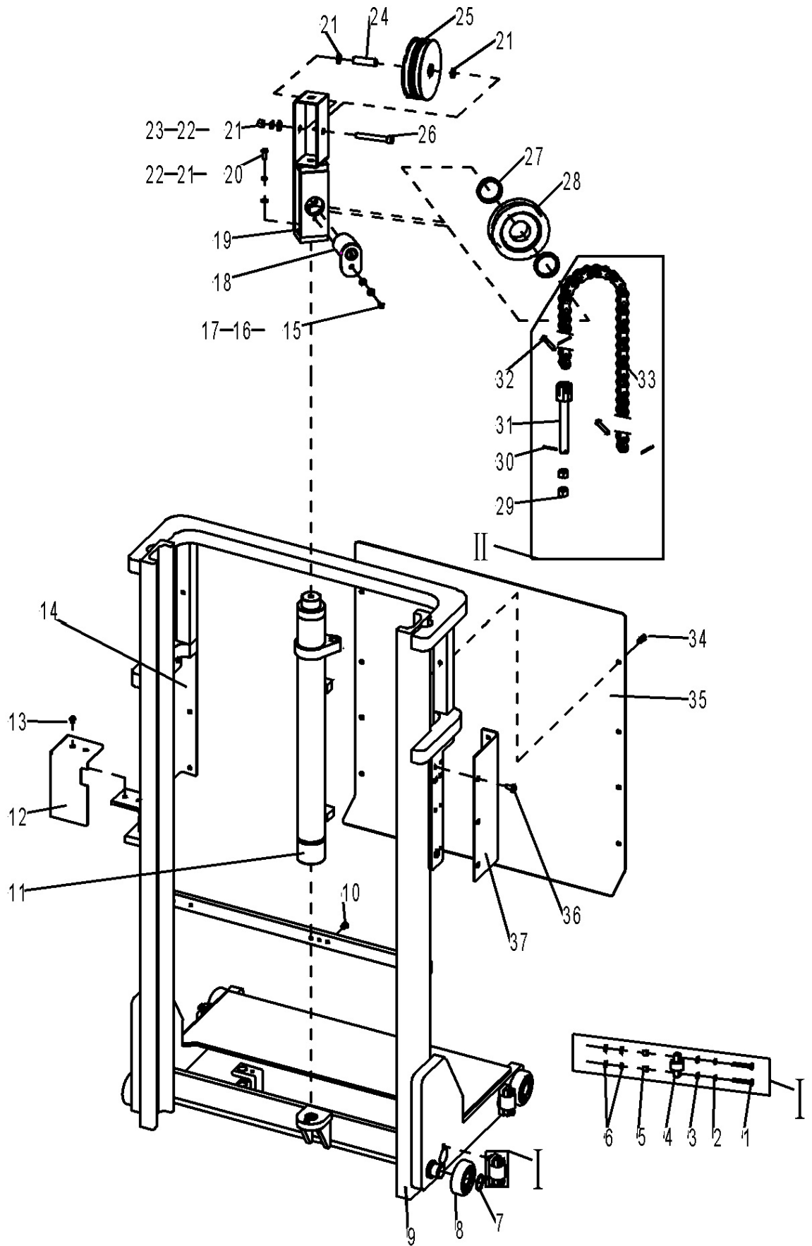
Fig. 12 Outer mast kits (single mast)
