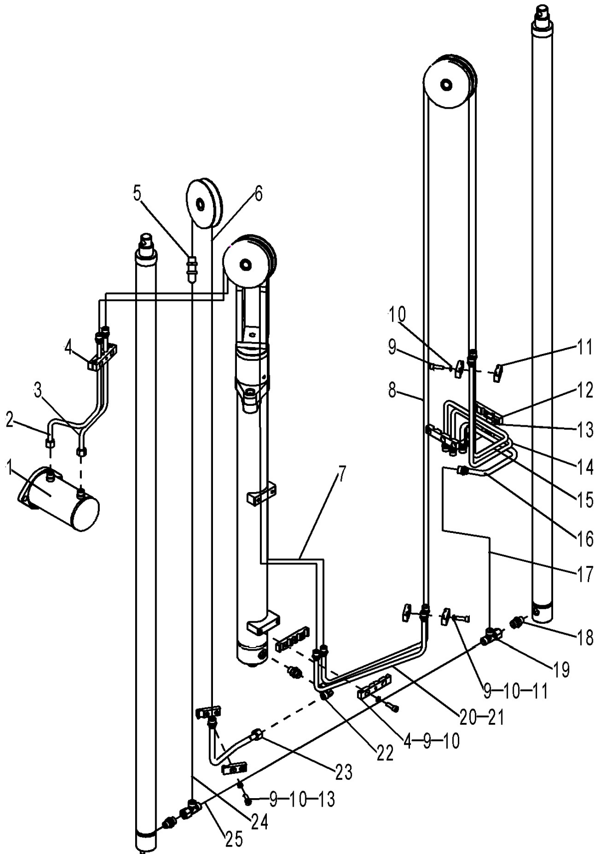
Fig. 21 Three stage mast hydraulic pipeline (three ways)
