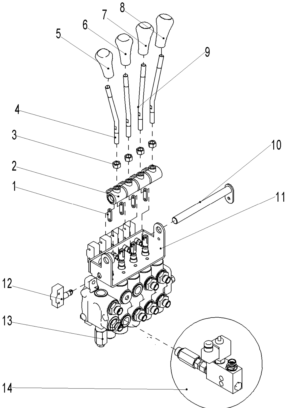
Fig. 41 Multi tandem valve (four ways)
