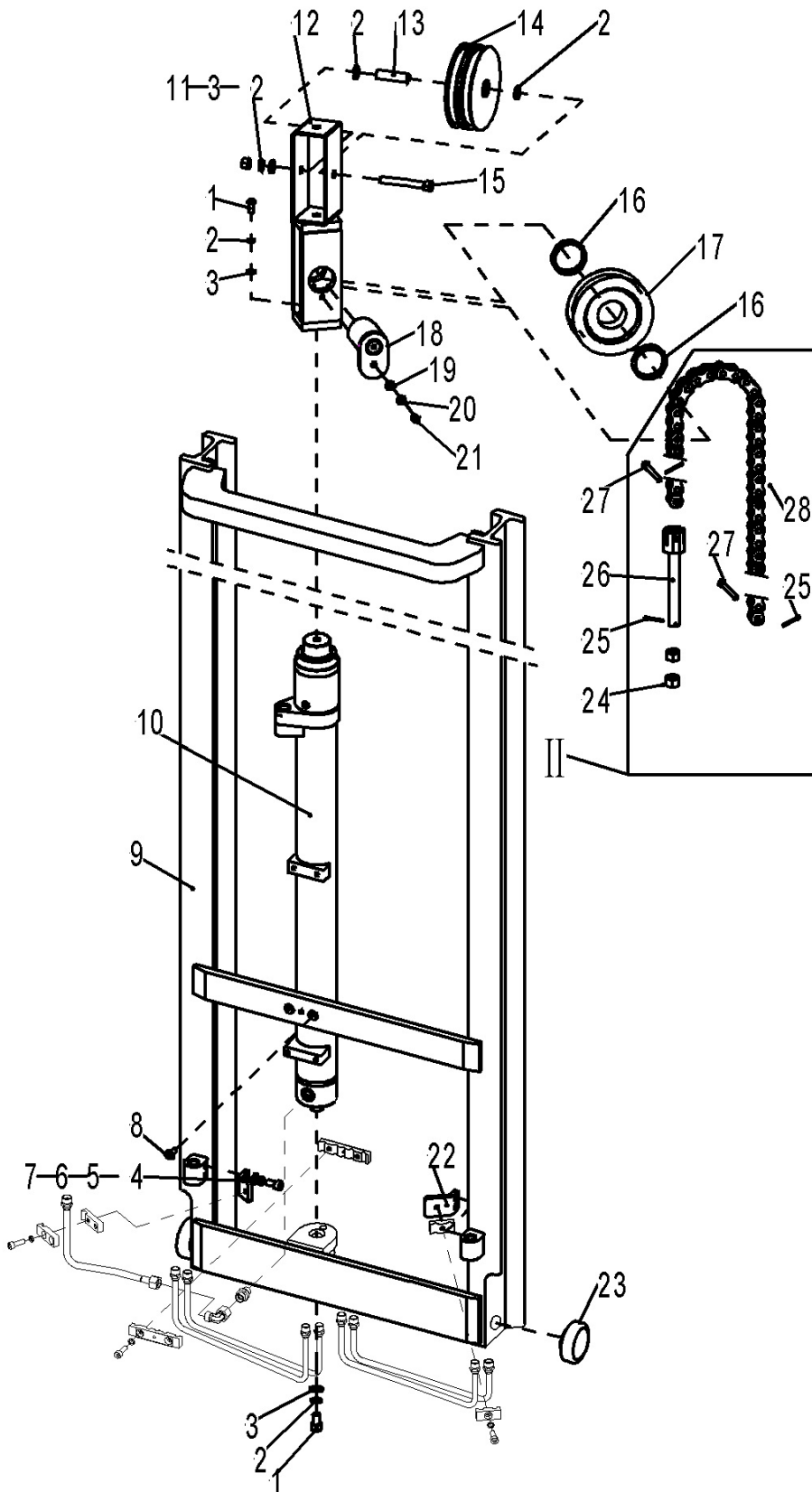
Fig. 16 Inner mast kits (three stage mast)
