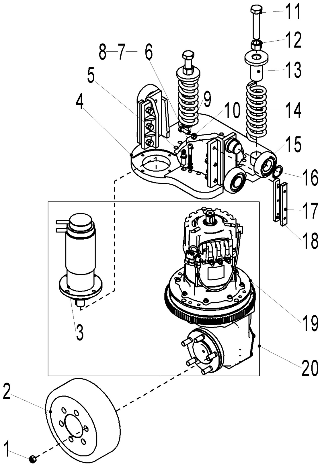
Fig. 23 Drive assembly
